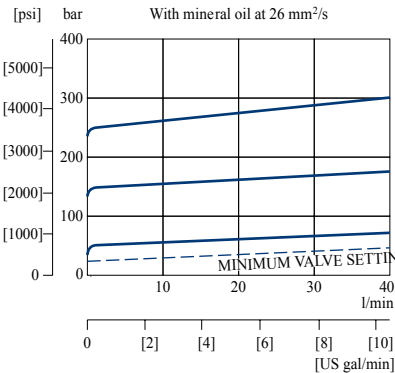
Pressure vs flow
