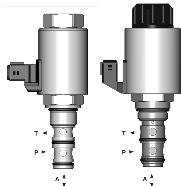
Directly operated reducing-relieving valves PVRM1-063 and PVRM3-10 with a metric connecting thread.
