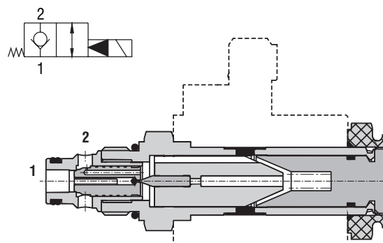
Screw-in cartridge poppet valve, pilot operated
