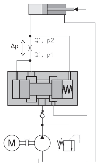
3-way pressure compensator
