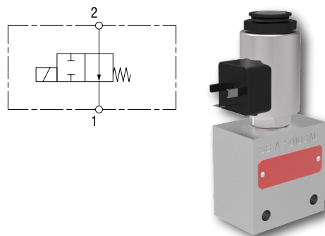
2-way, screw-in cartridge directional control valve SD2E-A2 in SB manifold used in an in-line design
